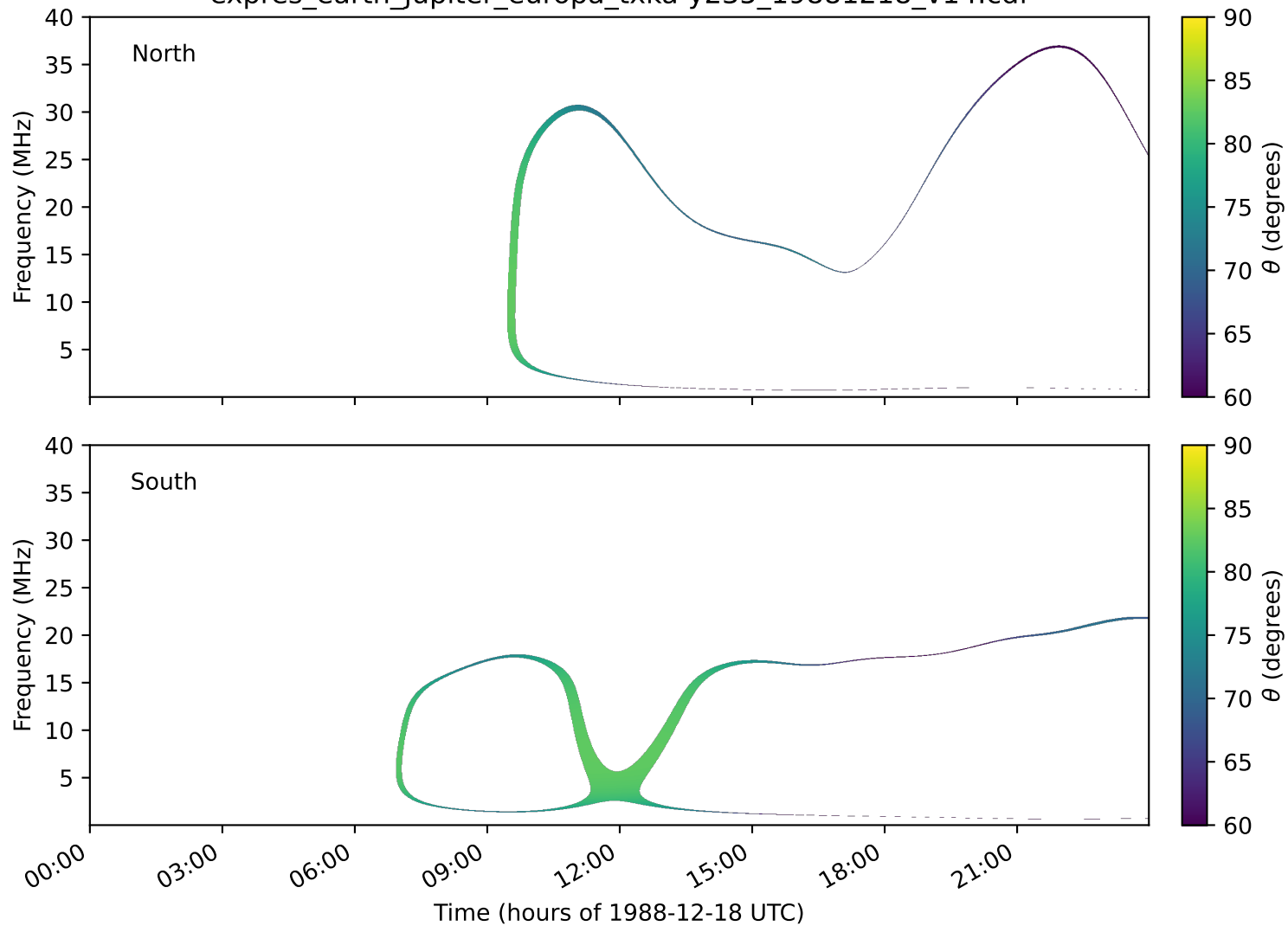
expres_earth_jupiter_europa_txka-y235_19881218_v14.cdf
