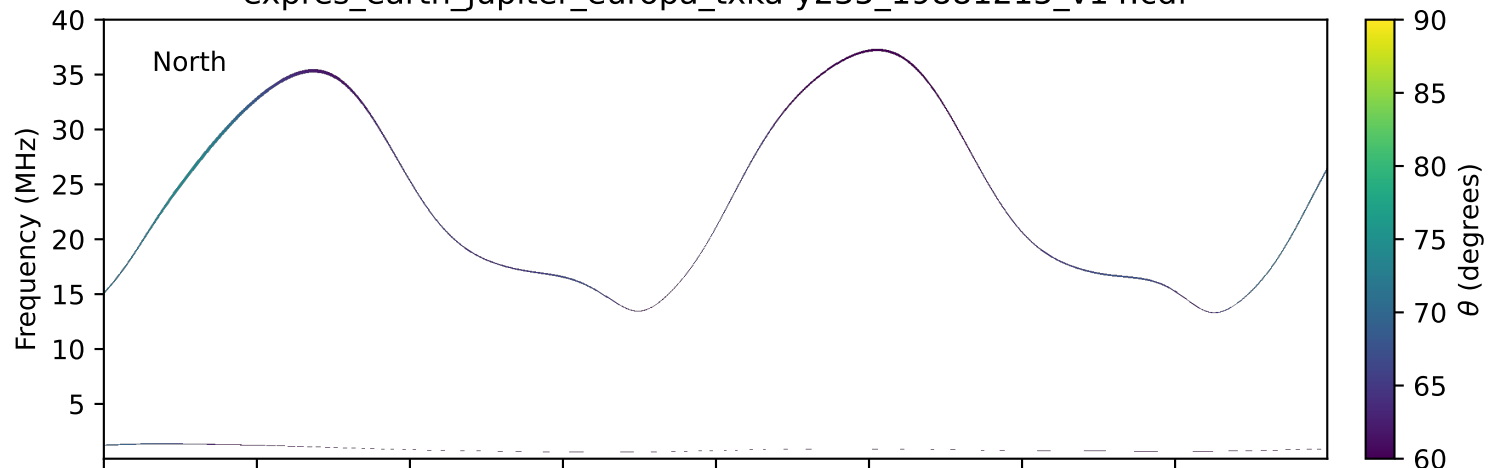
expres_earth_jupiter_europa_txka-y235_19881215_v14.cdf
