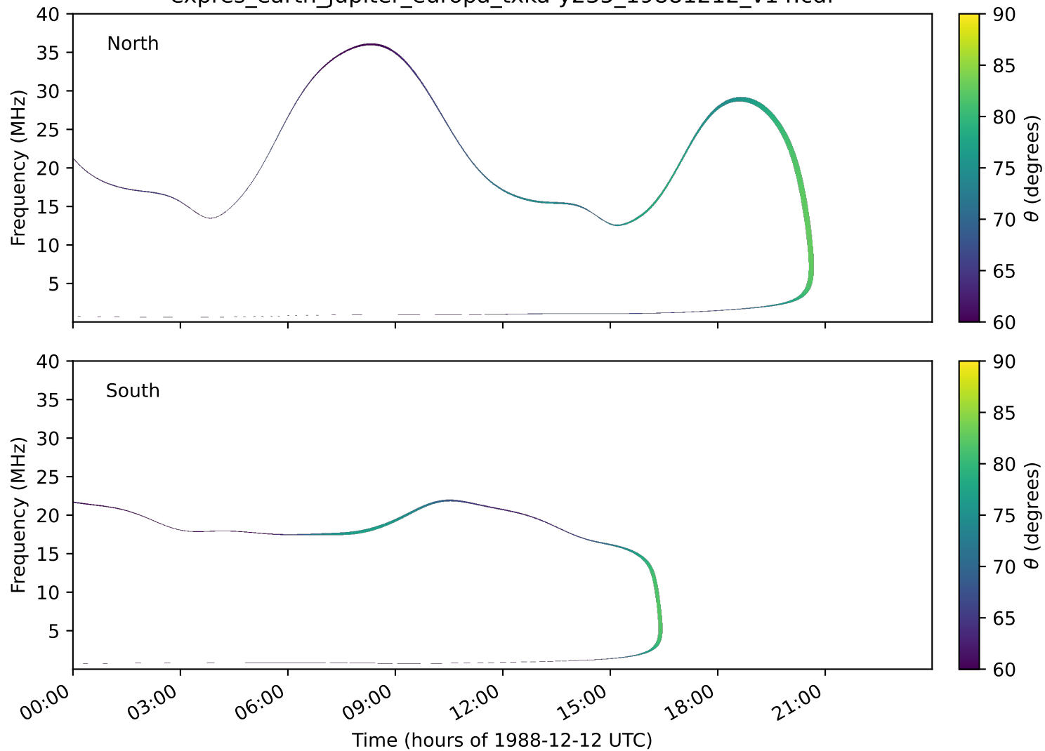
expres_earth_jupiter_europa_txka-y235_19881212_v14.cdf
