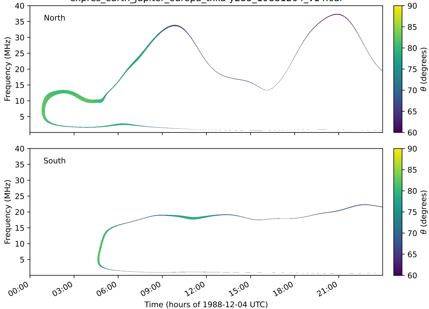
expres_earth_jupiter_europa_txka-y235_19881204_v14.cdf
