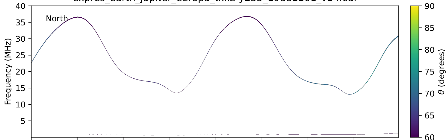
expres_earth_jupiter_europa_txka-y235_19881201_v14.cdf
