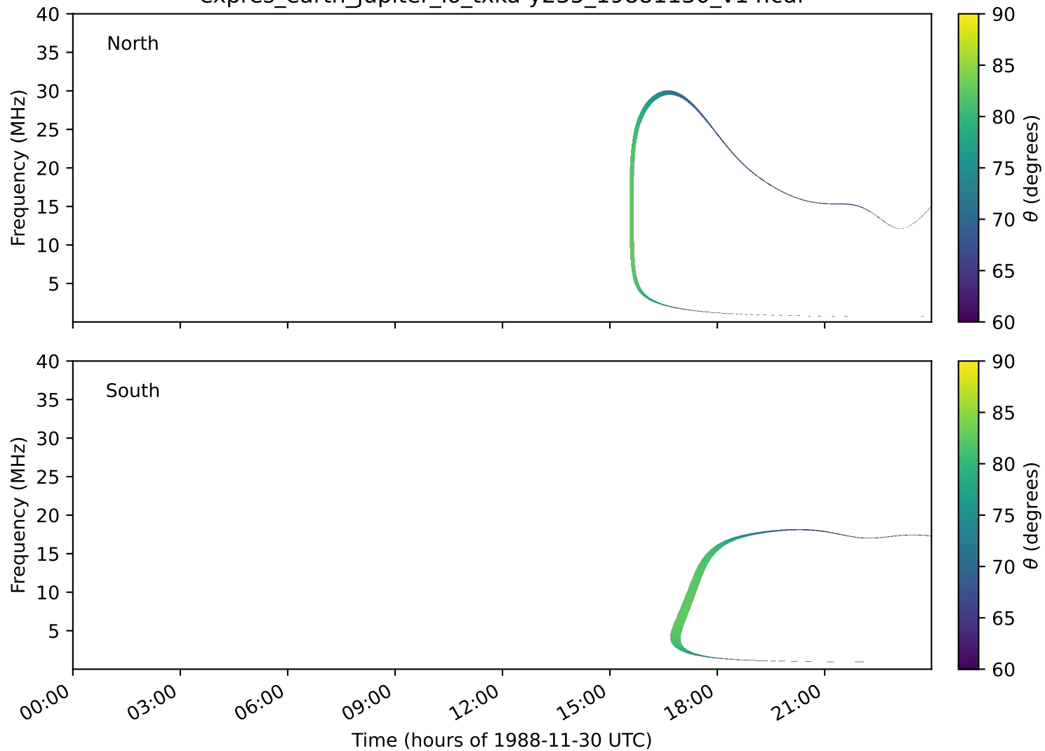
expres_earth_jupiter_io_txka-y235_19881130_v14.cdf
