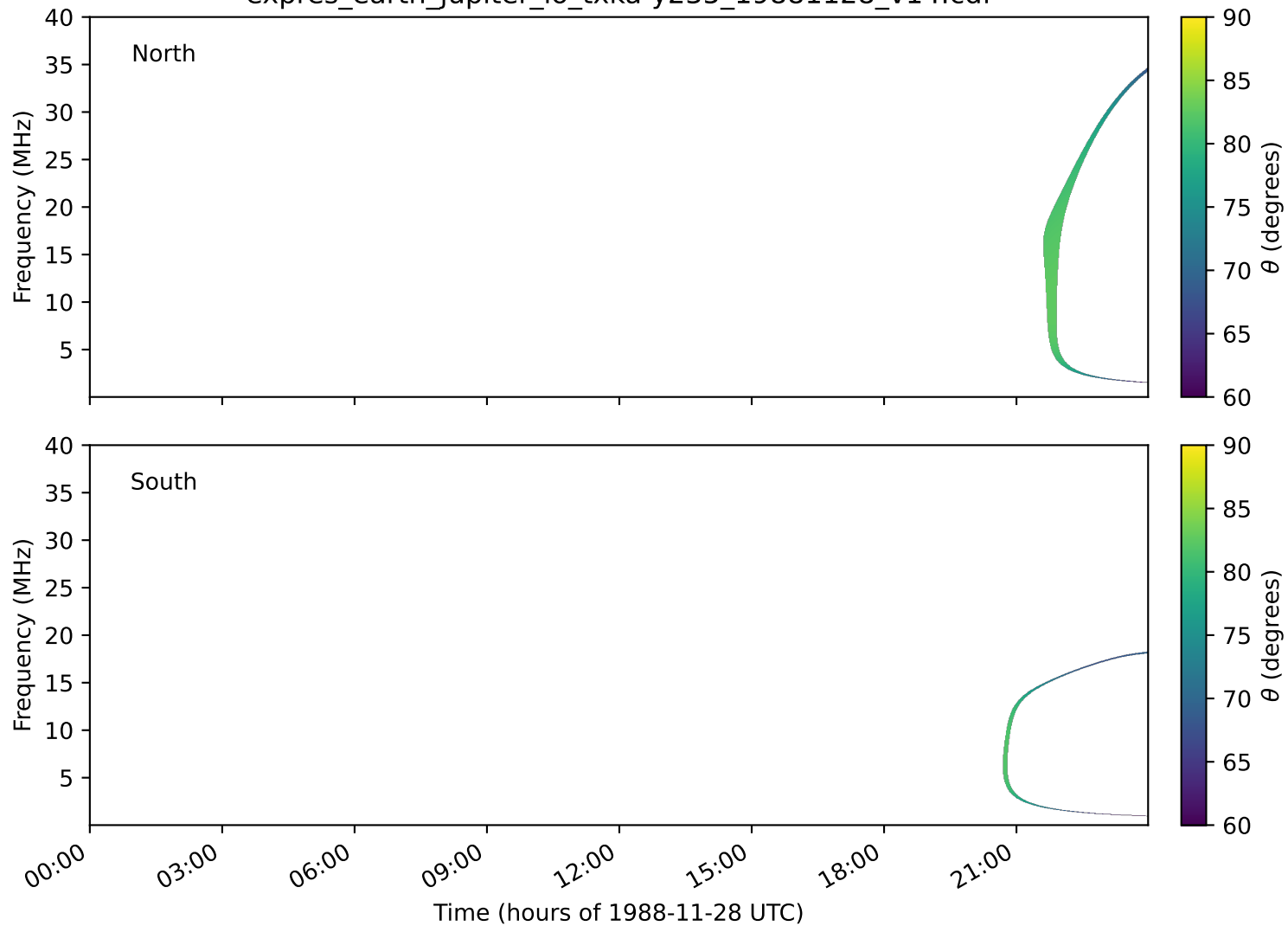
expres_earth_jupiter_io_txka-y235_19881128_v14.cdf
