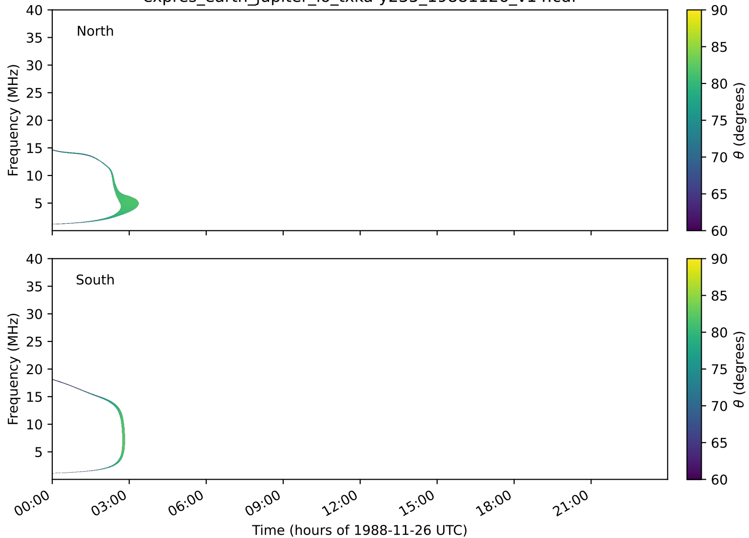
expres_earth_jupiter_io_txka-y235_19881126_v14.cdf
