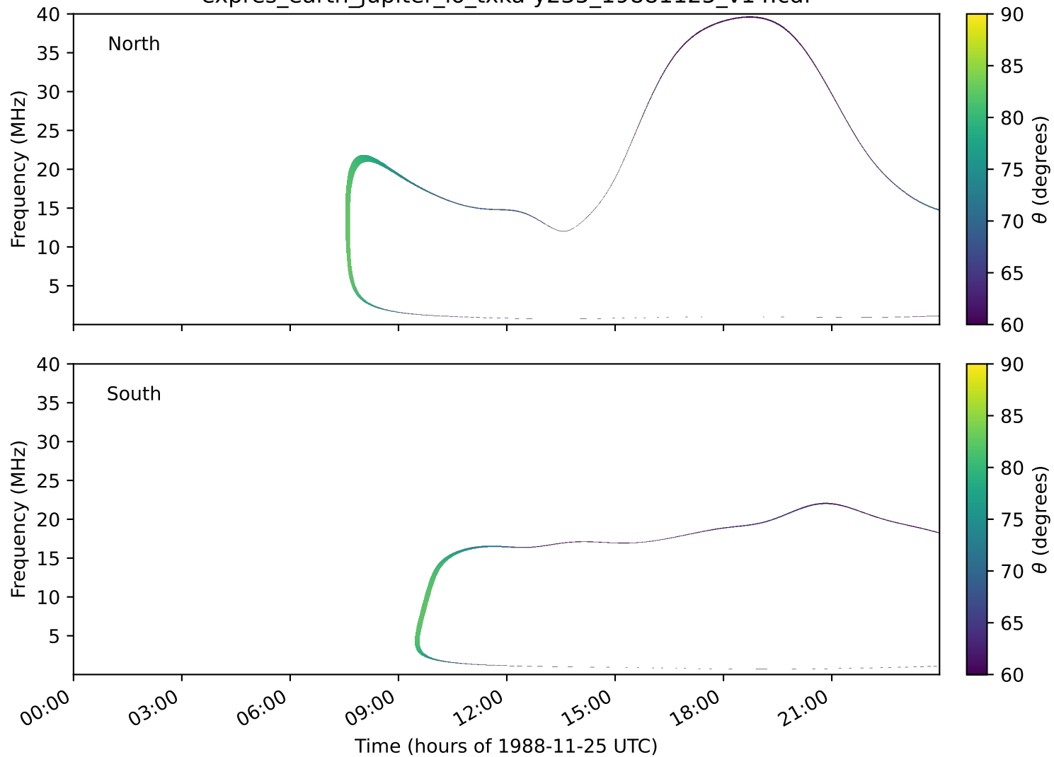
expres_earth_jupiter_io_txka-y235_19881125_v14.cdf
