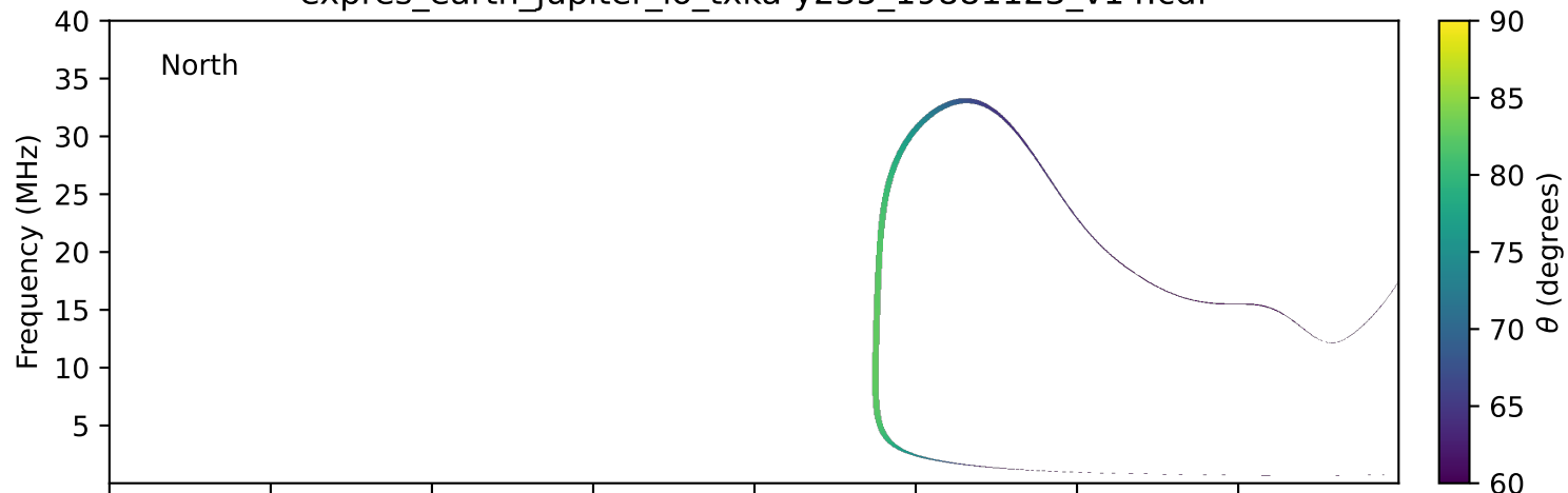
expres_earth_jupiter_io_txka-y235_19881123_v14.cdf
