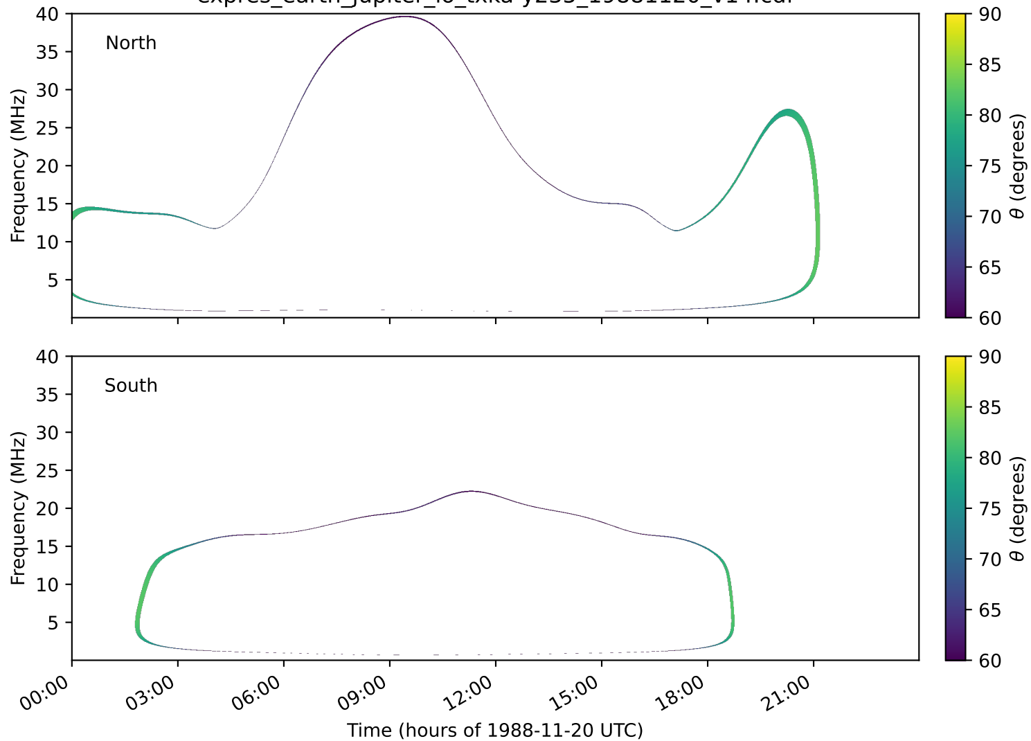
expres_earth_jupiter_io_txka-y235_19881120_v14.cdf
