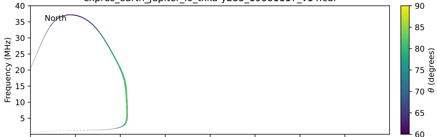
expres_earth_jupiter_io_txka-y235_19881117_v14.cdf
