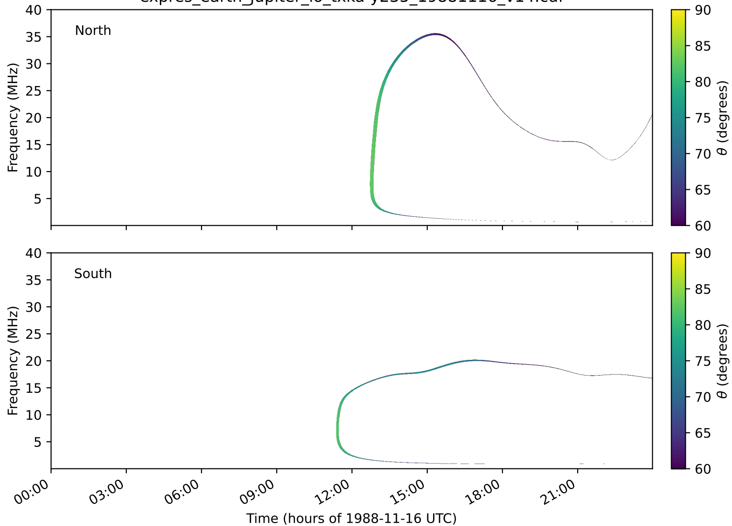
expres_earth_jupiter_io_txka-y235_19881116_v14.cdf
