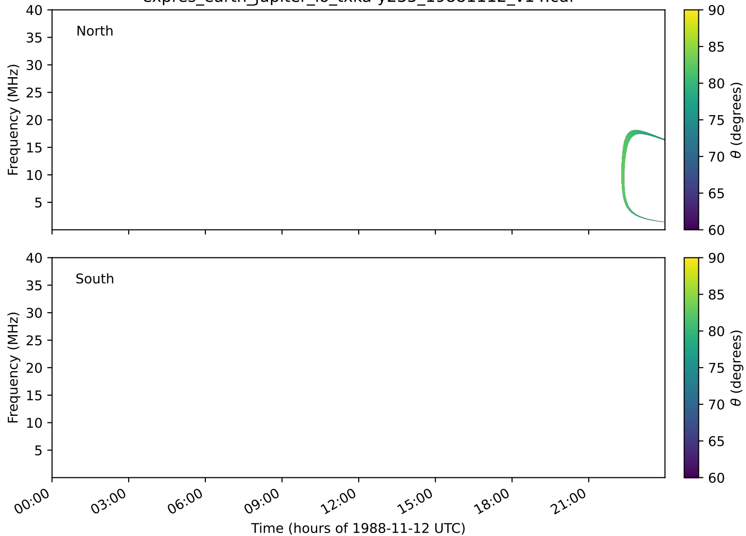
expres_earth_jupiter_io_txka-y235_19881112_v14.cdf
