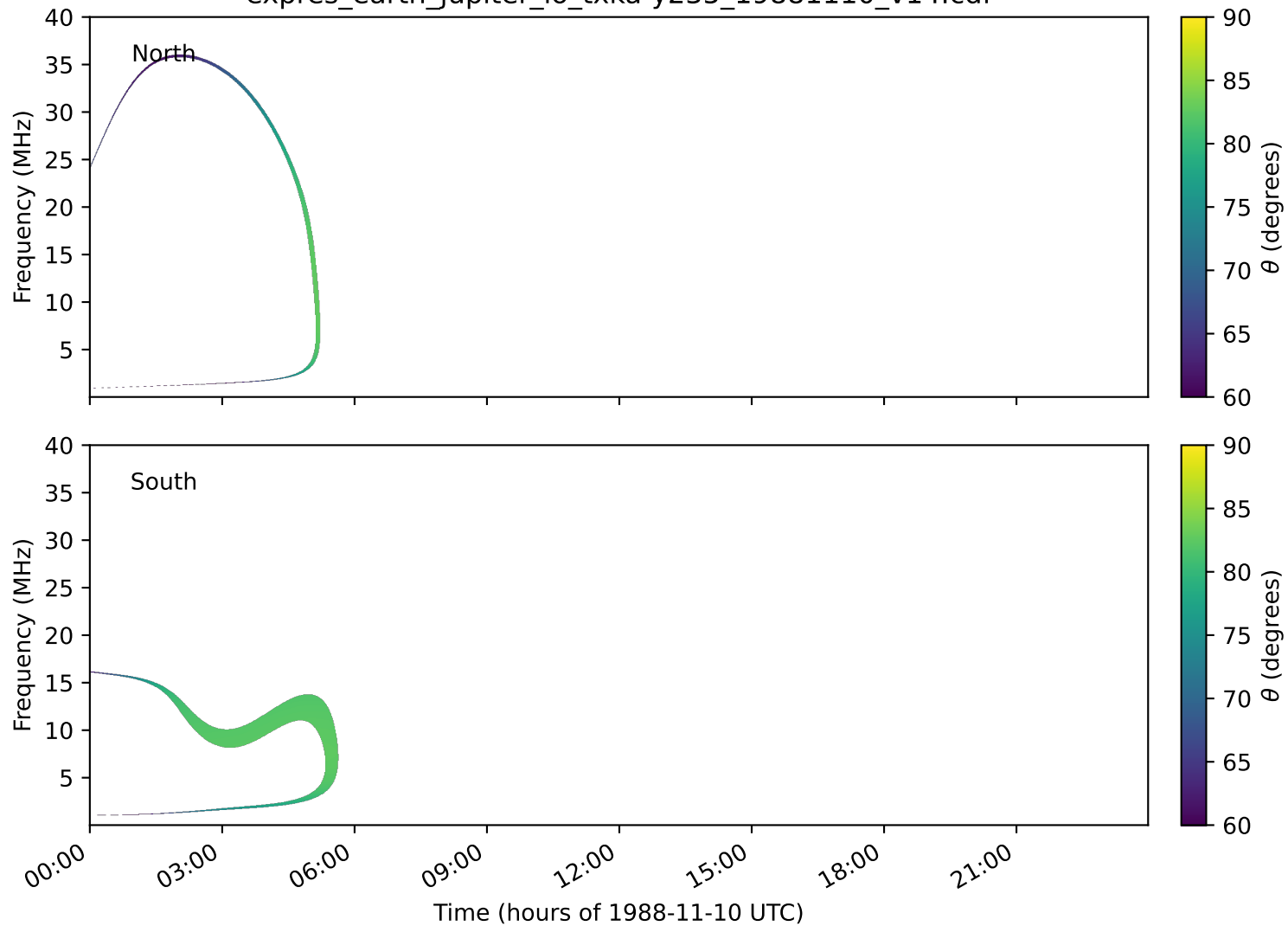
expres_earth_jupiter_io_txka-y235_19881110_v14.cdf
