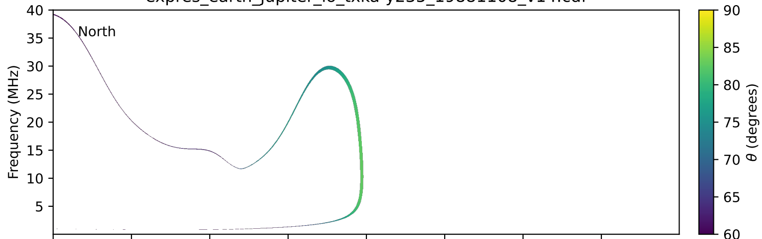
expres_earth_jupiter_io_txka-y235_19881108_v14.cdf
