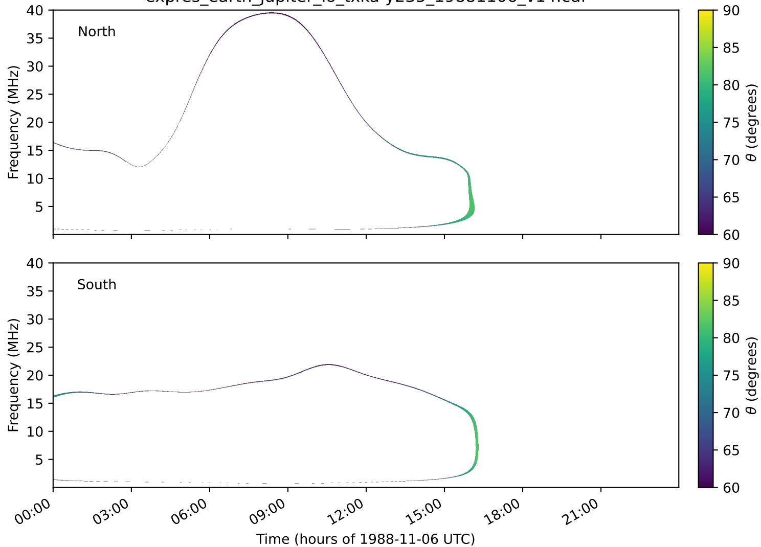
expres_earth_jupiter_io_txka-y235_19881106_v14.cdf
