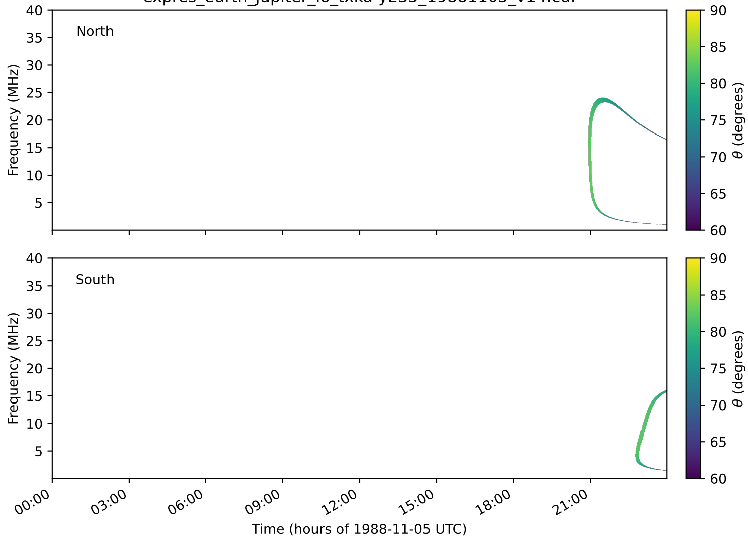
expres_earth_jupiter_io_txka-y235_19881105_v14.cdf
