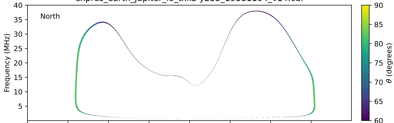
expres_earth_jupiter_io_txka-y235_19881104_v14.cdf
