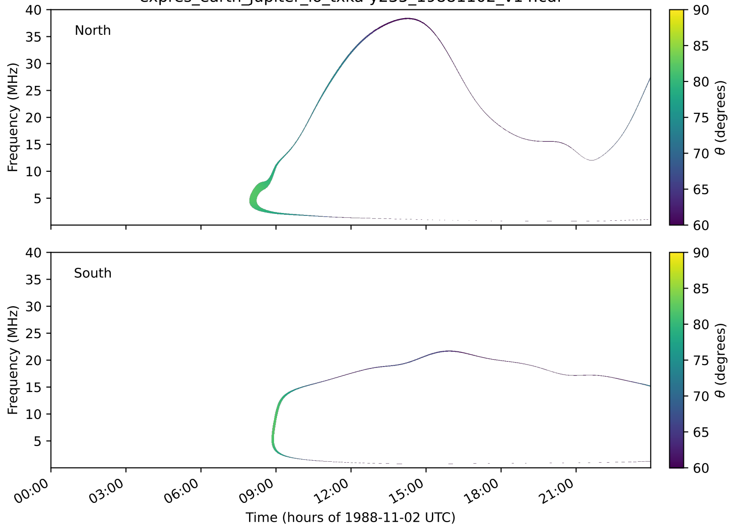
expres_earth_jupiter_io_txka-y235_19881102_v14.cdf
