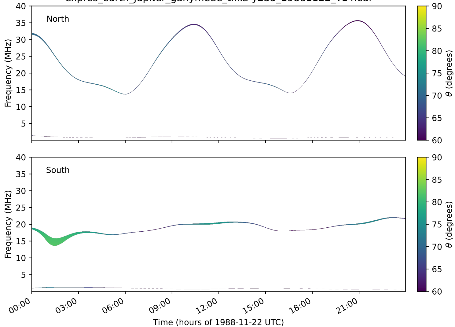
expres_earth_jupiter_ganymede_txka-y235_19881122_v14.cdf
