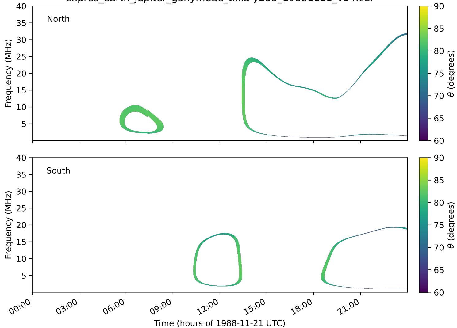
expres_earth_jupiter_ganymede_txka-y235_19881121_v14.cdf
