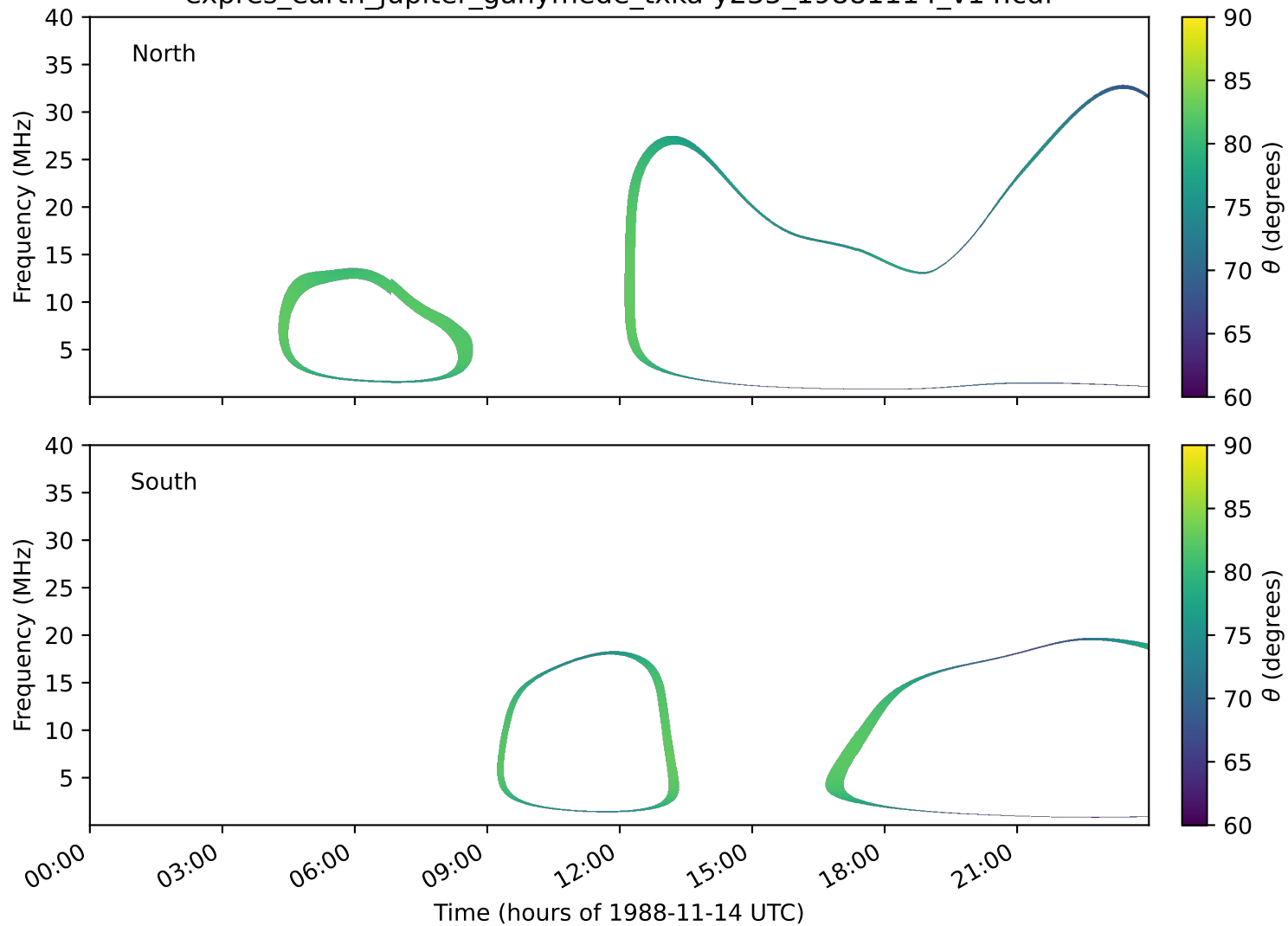
expres_earth_jupiter_ganymede_txka-y235_19881114_v14.cdf
