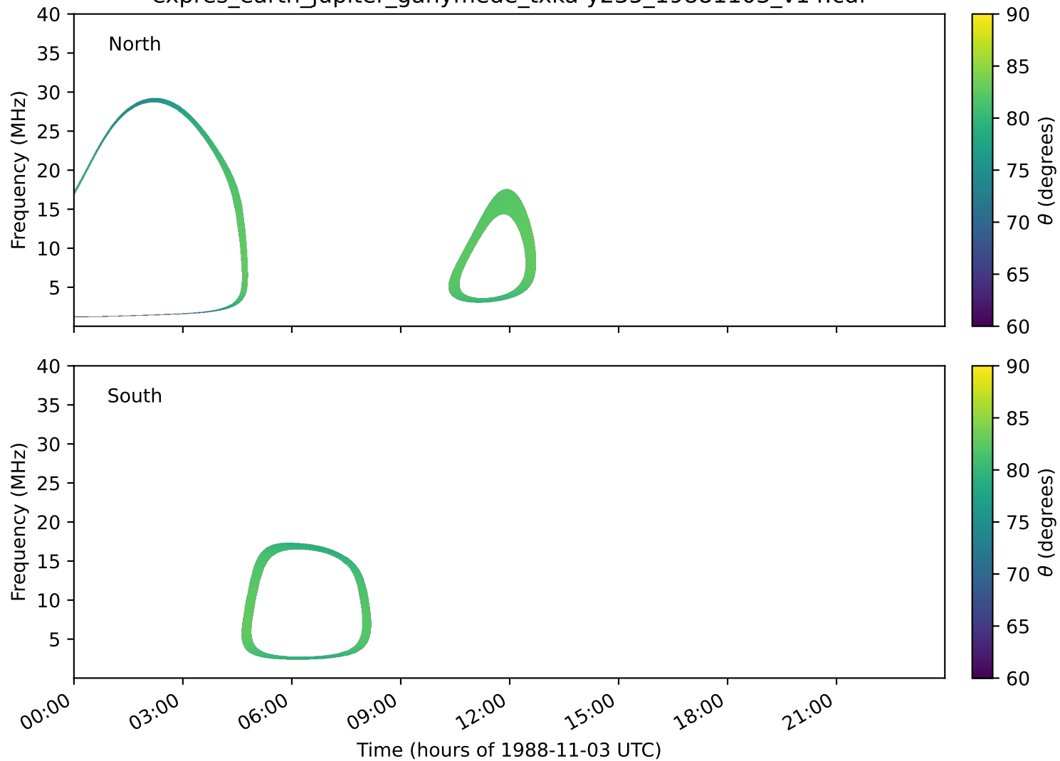
expres_earth_jupiter_ganymede_txka-y235_19881103_v14.cdf
