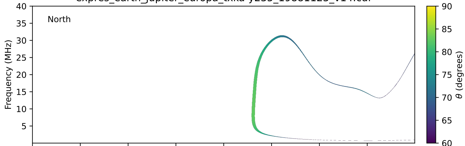
expres_earth_jupiter_europa_txka-y235_19881123_v14.cdf
