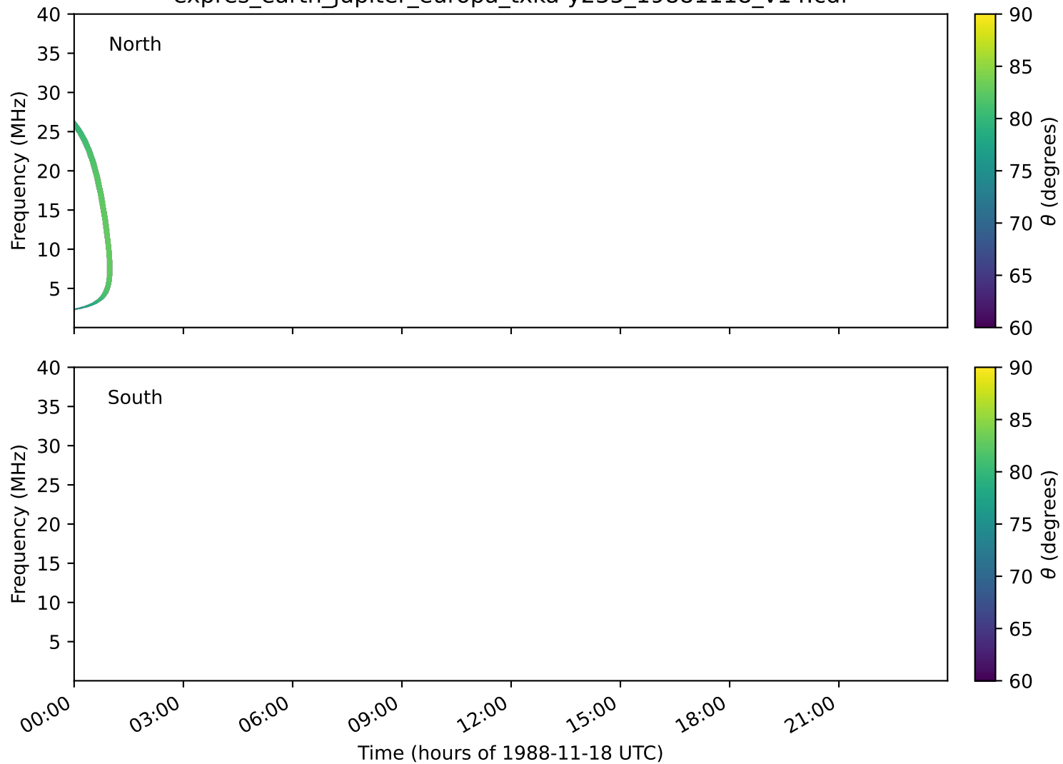
expres_earth_jupiter_europa_txka-y235_19881118_v14.cdf
