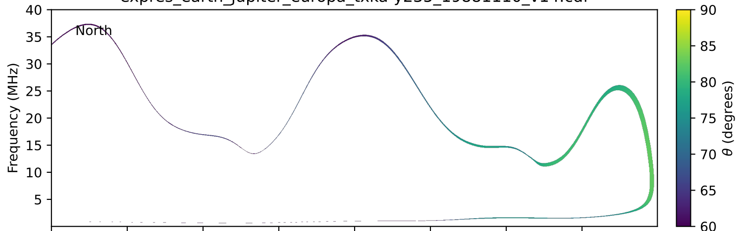
expres_earth_jupiter_europa_txka-y235_19881110_v14.cdf
