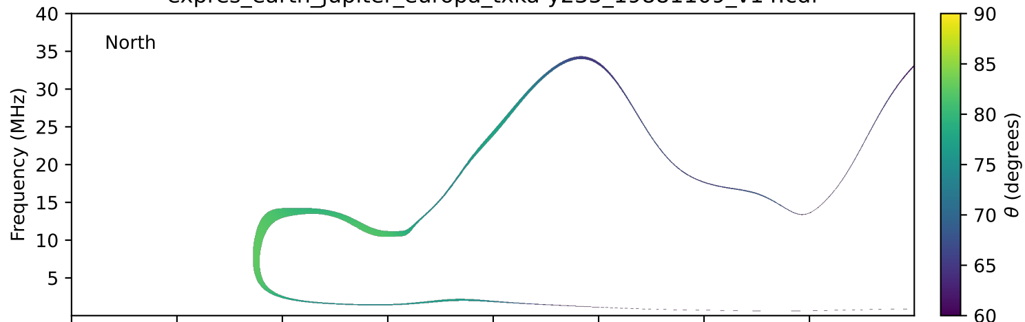
expres_earth_jupiter_europa_txka-y235_19881109_v14.cdf
