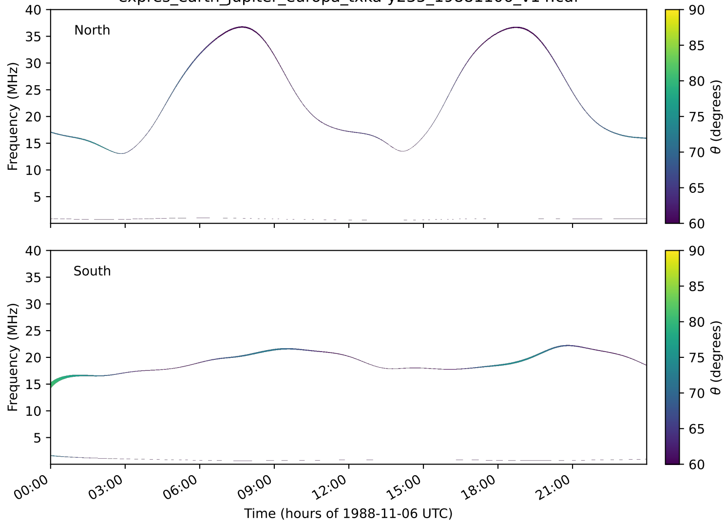
expres_earth_jupiter_europa_txka-y235_19881106_v14.cdf
