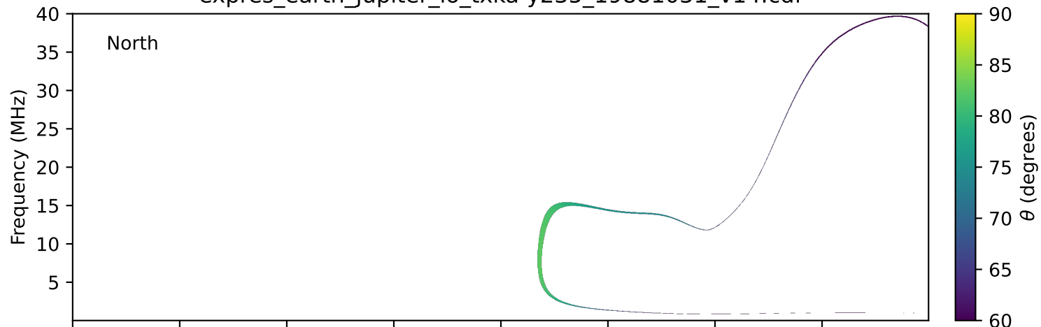
expres_earth_jupiter_io_txka-y235_19881031_v14.cdf
