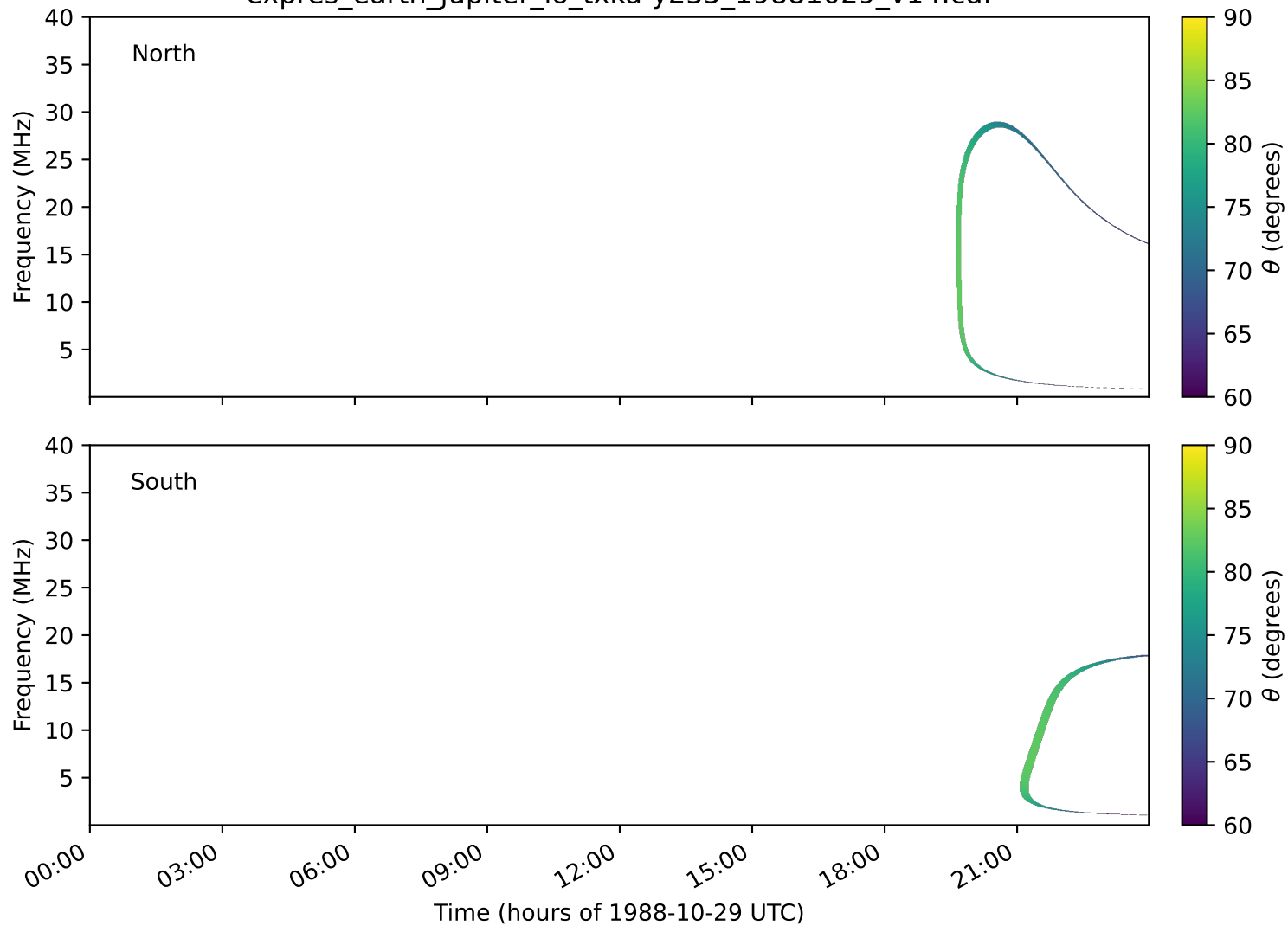
expres_earth_jupiter_io_txka-y235_19881029_v14.cdf
