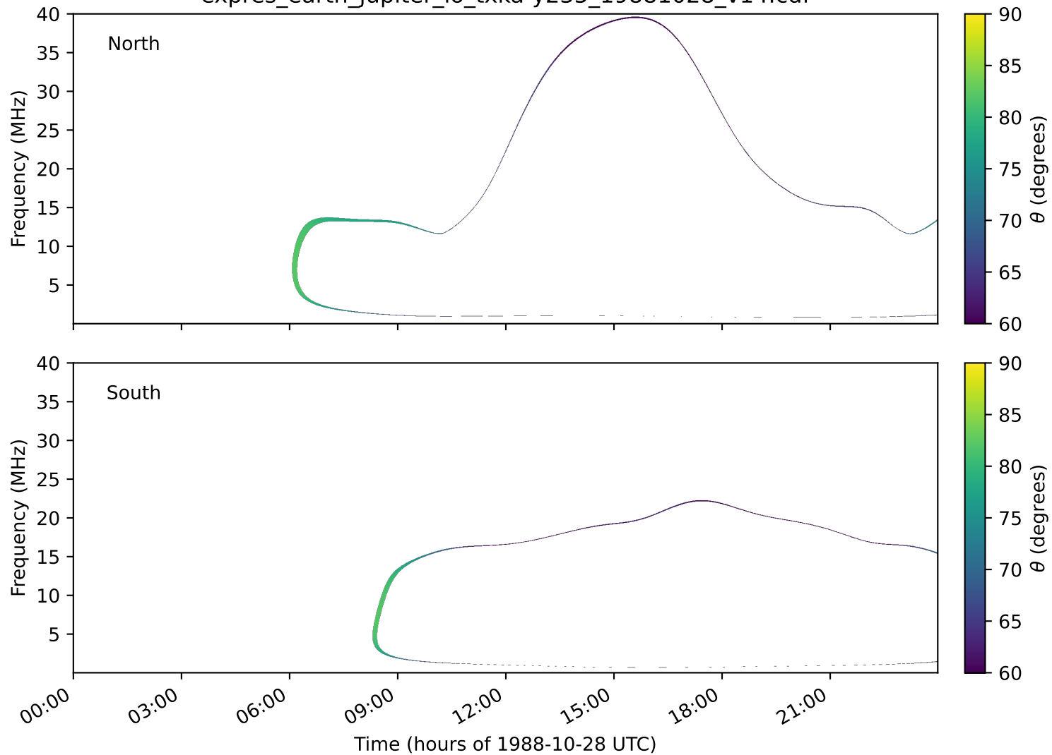
expres_earth_jupiter_io_txka-y235_19881028_v14.cdf
