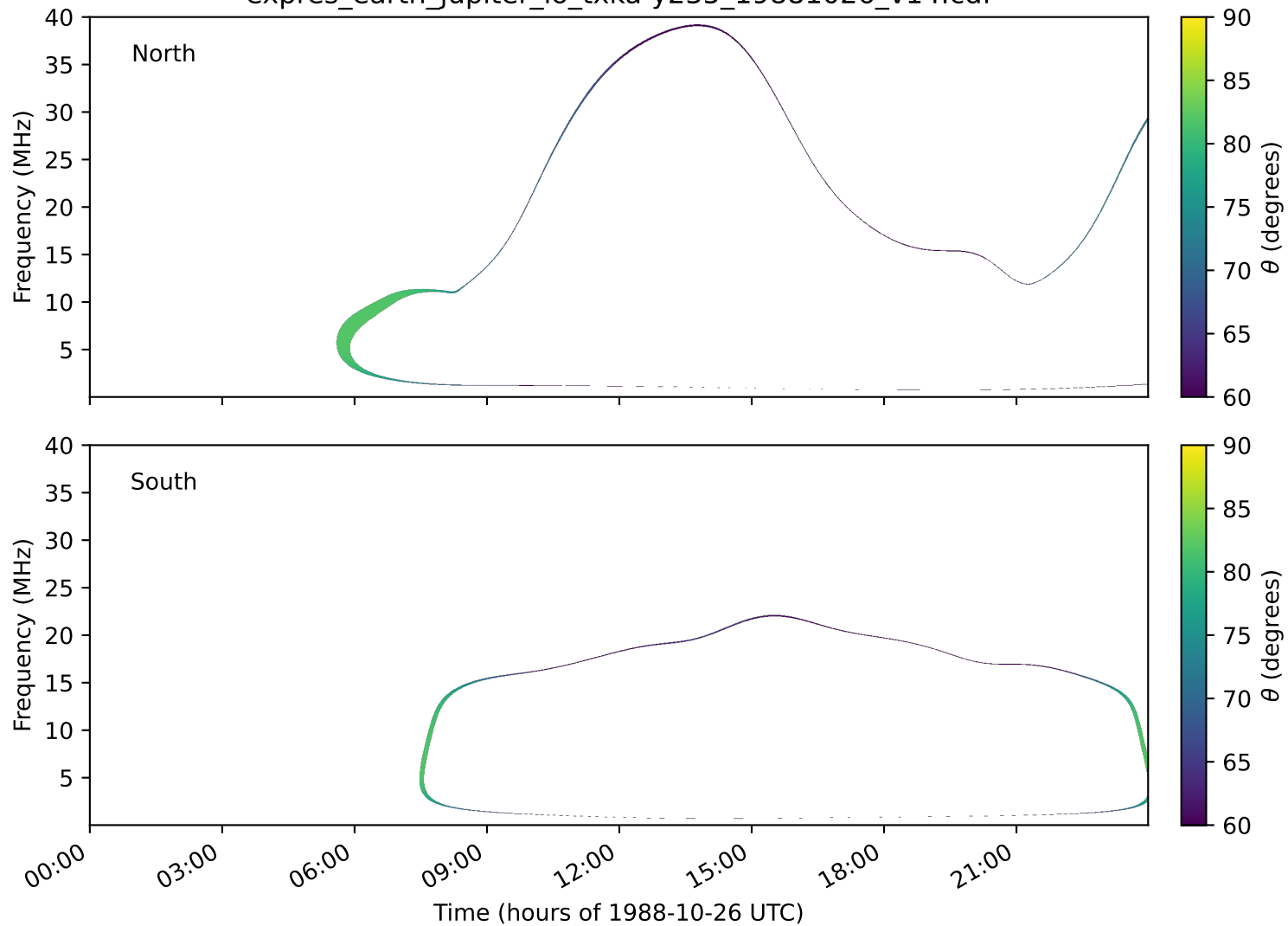
expres_earth_jupiter_io_txka-y235_19881026_v14.cdf
