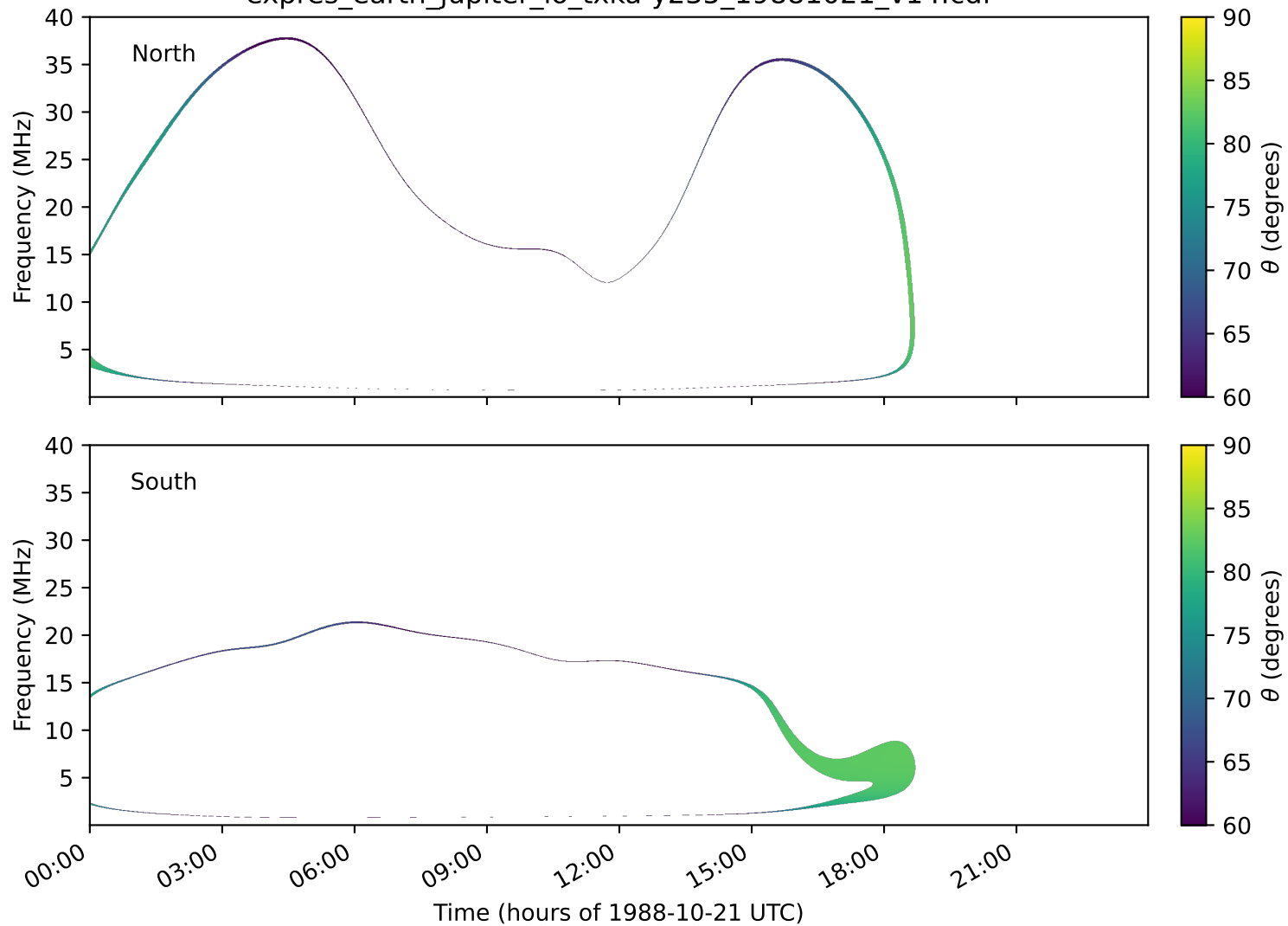
expres_earth_jupiter_io_txka-y235_19881021_v14.cdf
