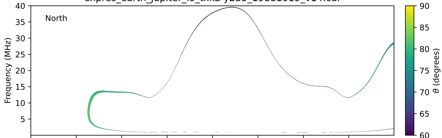
expres_earth_jupiter_io_txka-y235_19881019_v14.cdf
