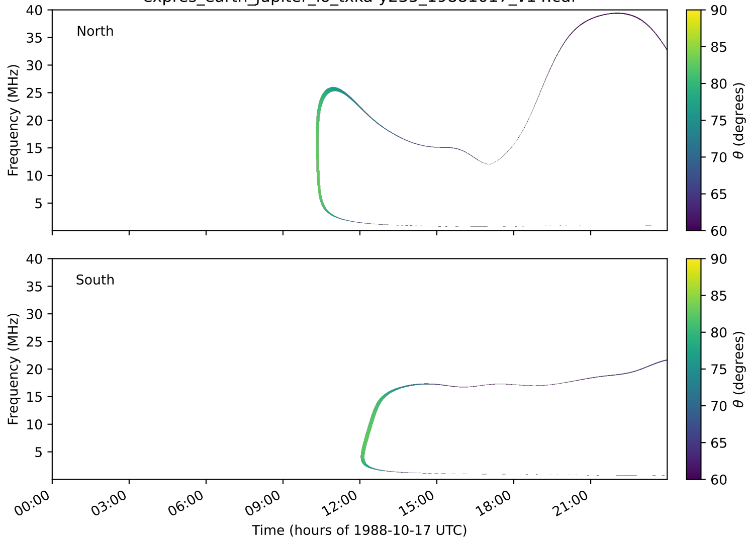
expres_earth_jupiter_io_txka-y235_19881017_v14.cdf
