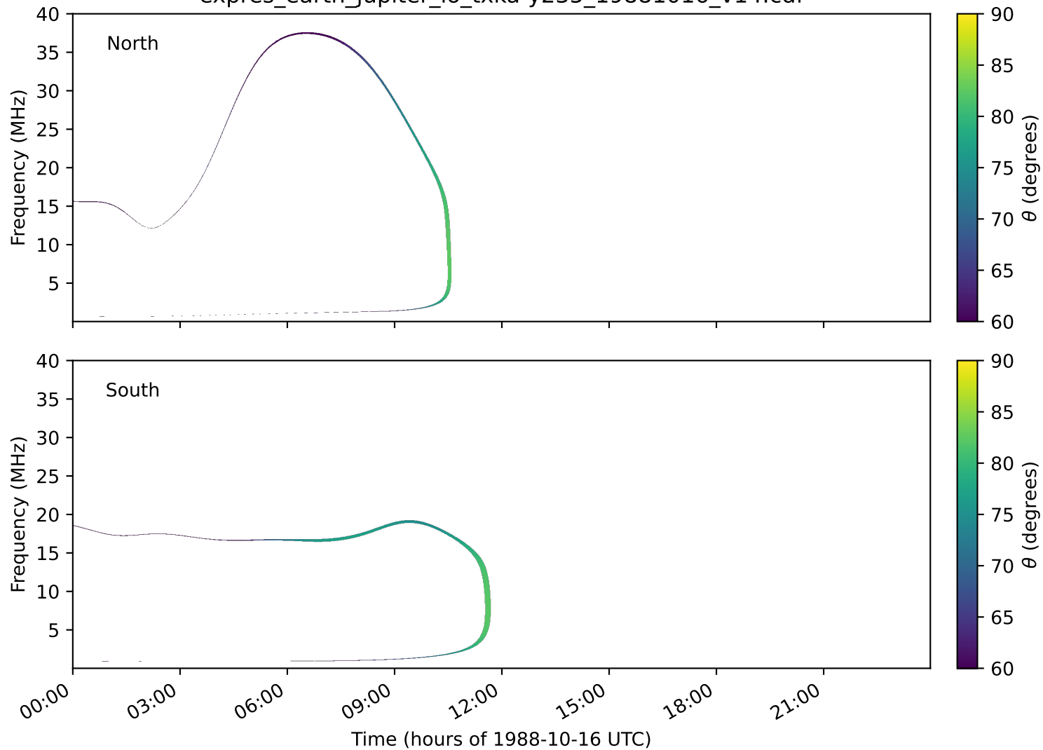
expres_earth_jupiter_io_txka-y235_19881016_v14.cdf
