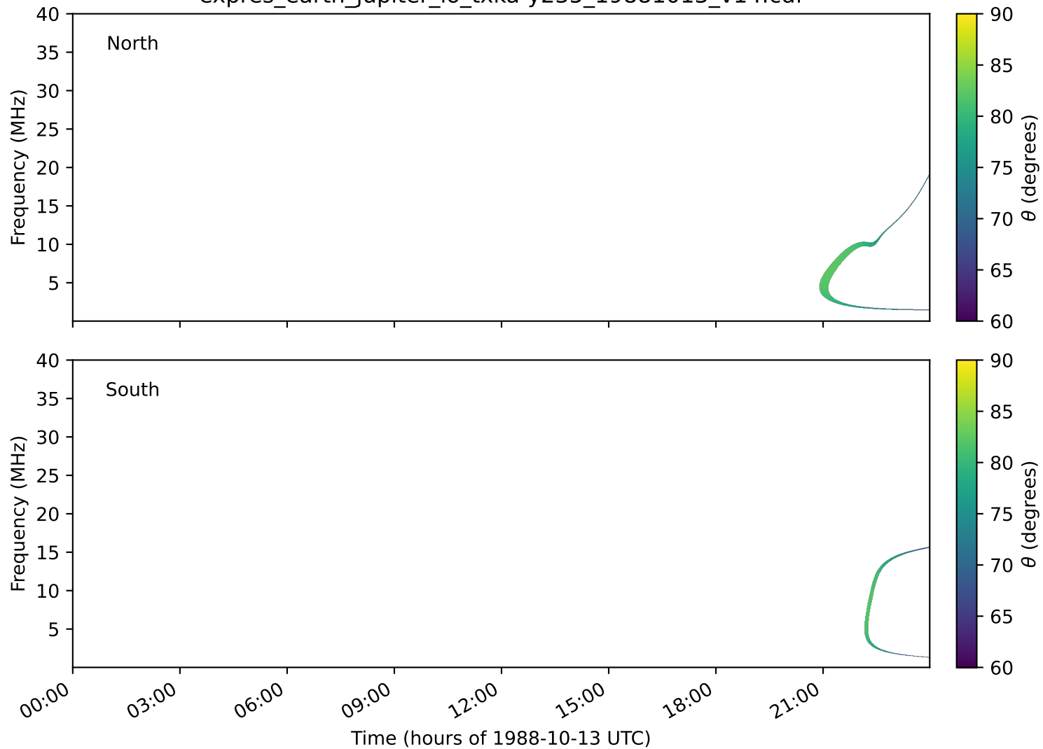
expres_earth_jupiter_io_txka-y235_19881013_v14.cdf
