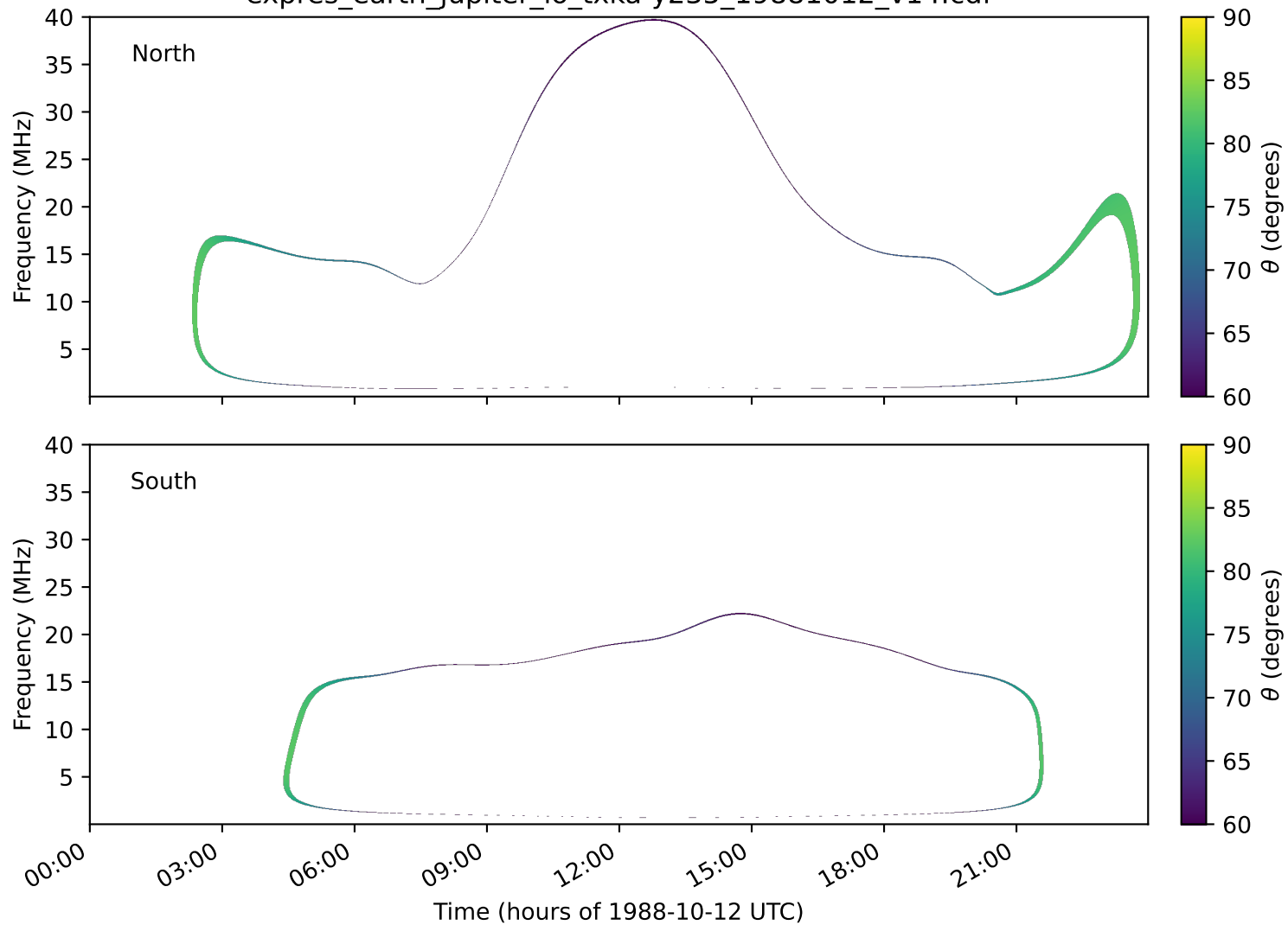
expres_earth_jupiter_io_txka-y235_19881012_v14.cdf
