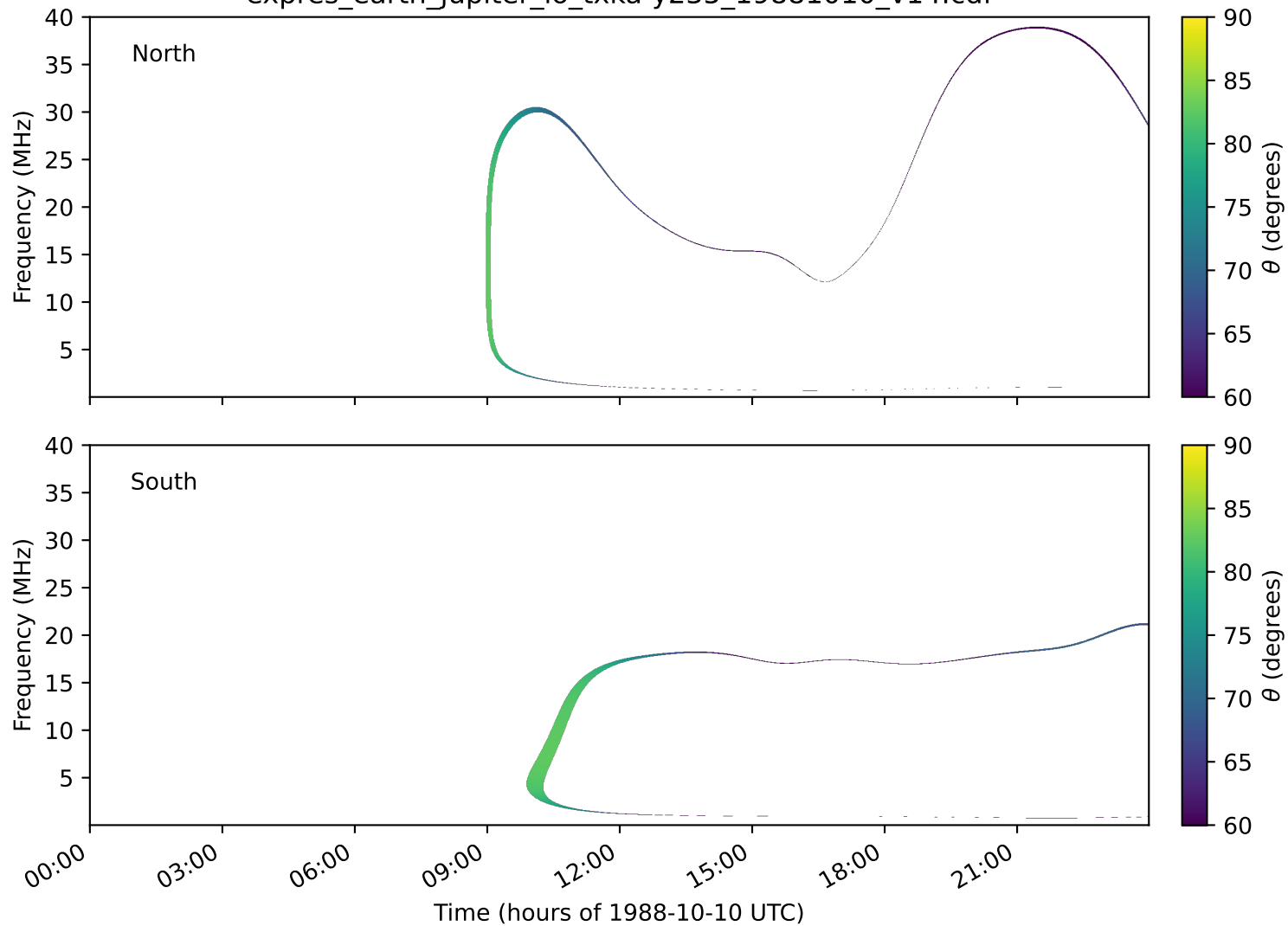
expres_earth_jupiter_io_txka-y235_19881010_v14.cdf
