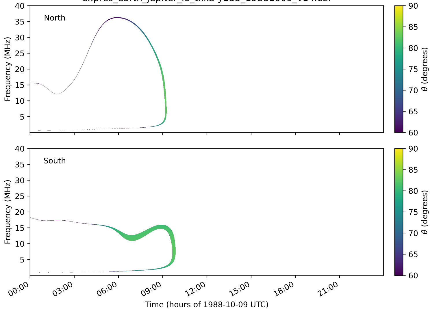
expres_earth_jupiter_io_txka-y235_19881009_v14.cdf
