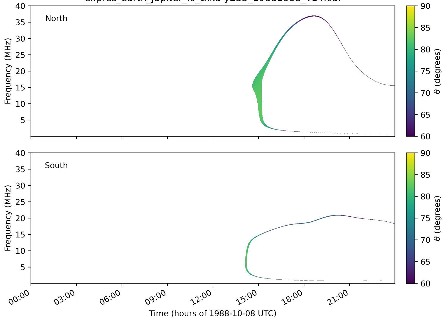
expres_earth_jupiter_io_txka-y235_19881008_v14.cdf
