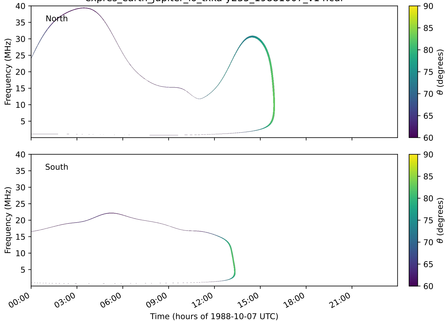
expres_earth_jupiter_io_txka-y235_19881007_v14.cdf
