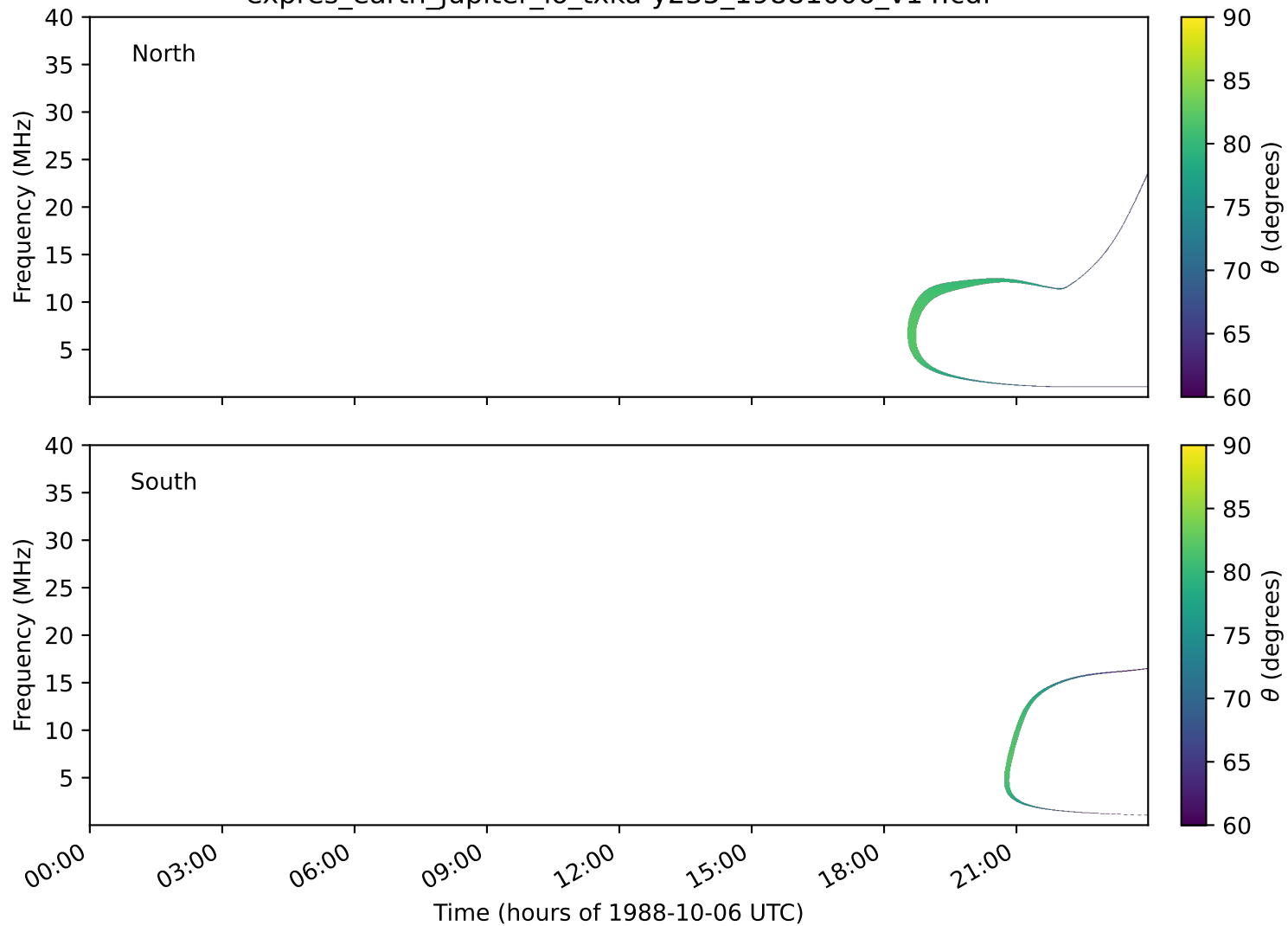
expres_earth_jupiter_io_txka-y235_19881006_v14.cdf
