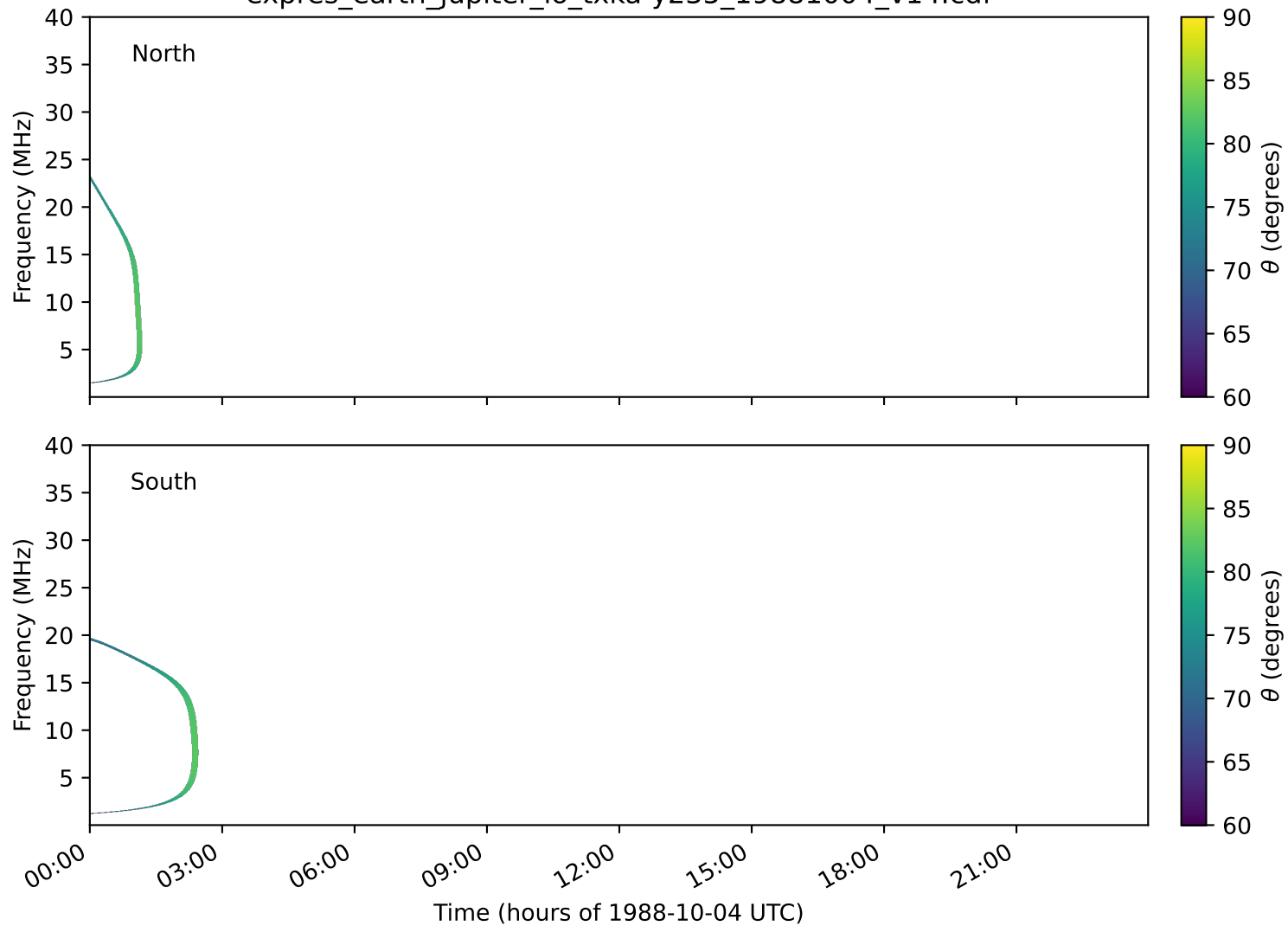
expres_earth_jupiter_io_txka-y235_19881004_v14.cdf
