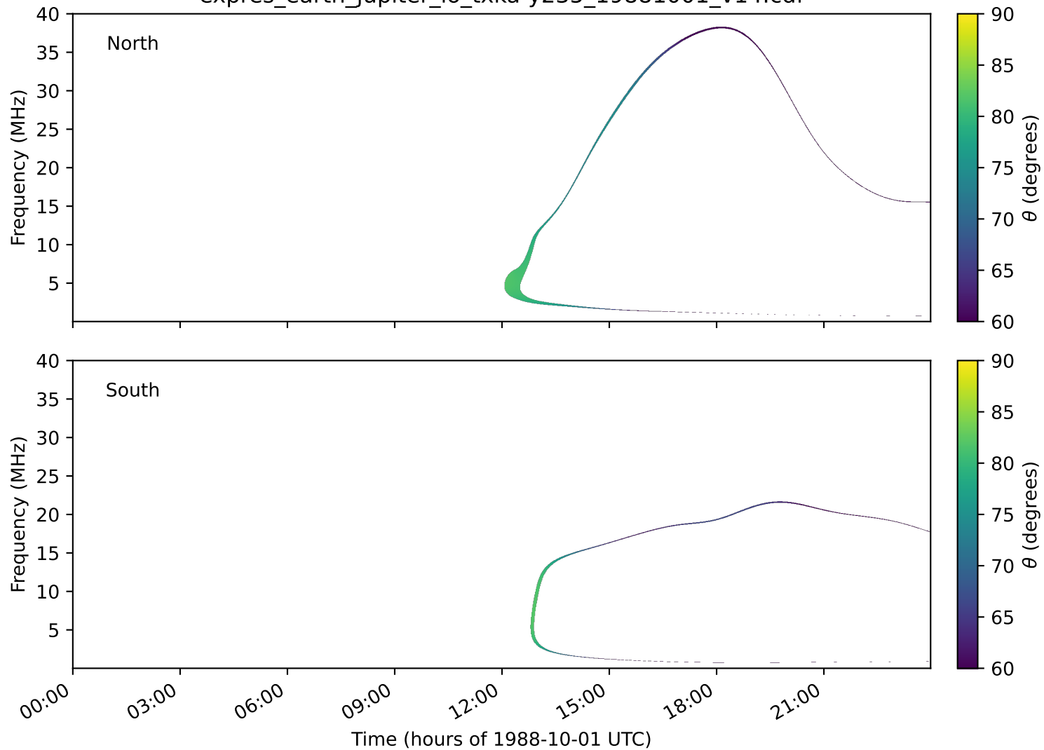
expres_earth_jupiter_io_txka-y235_19881001_v14.cdf
