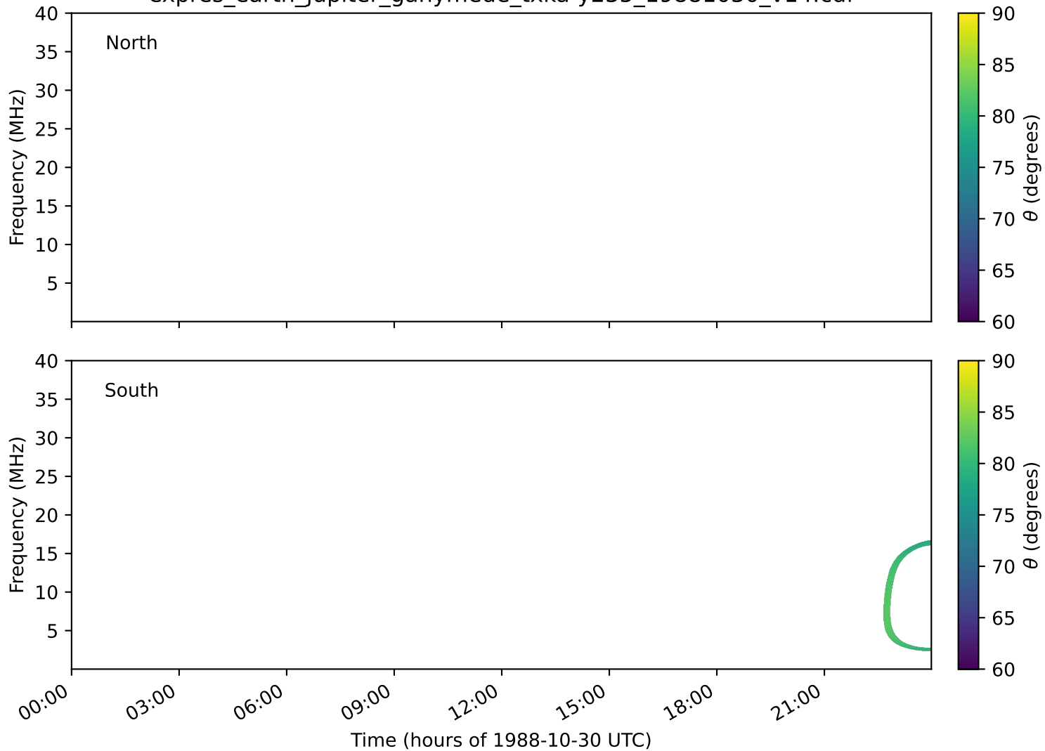
expres_earth_jupiter_ganymede_txka-y235_19881030_v14.cdf
