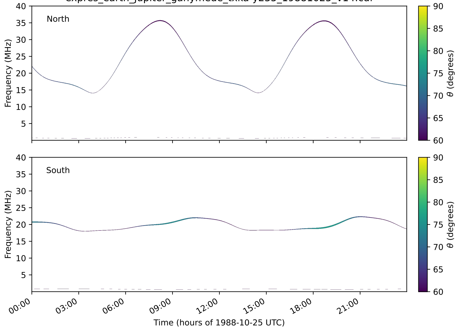
expres_earth_jupiter_ganymede_txka-y235_19881025_v14.cdf
