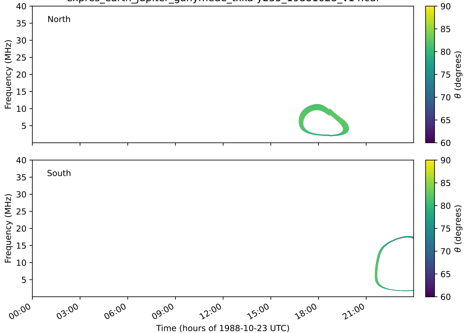
expres_earth_jupiter_ganymede_txka-y235_19881023_v14.cdf
