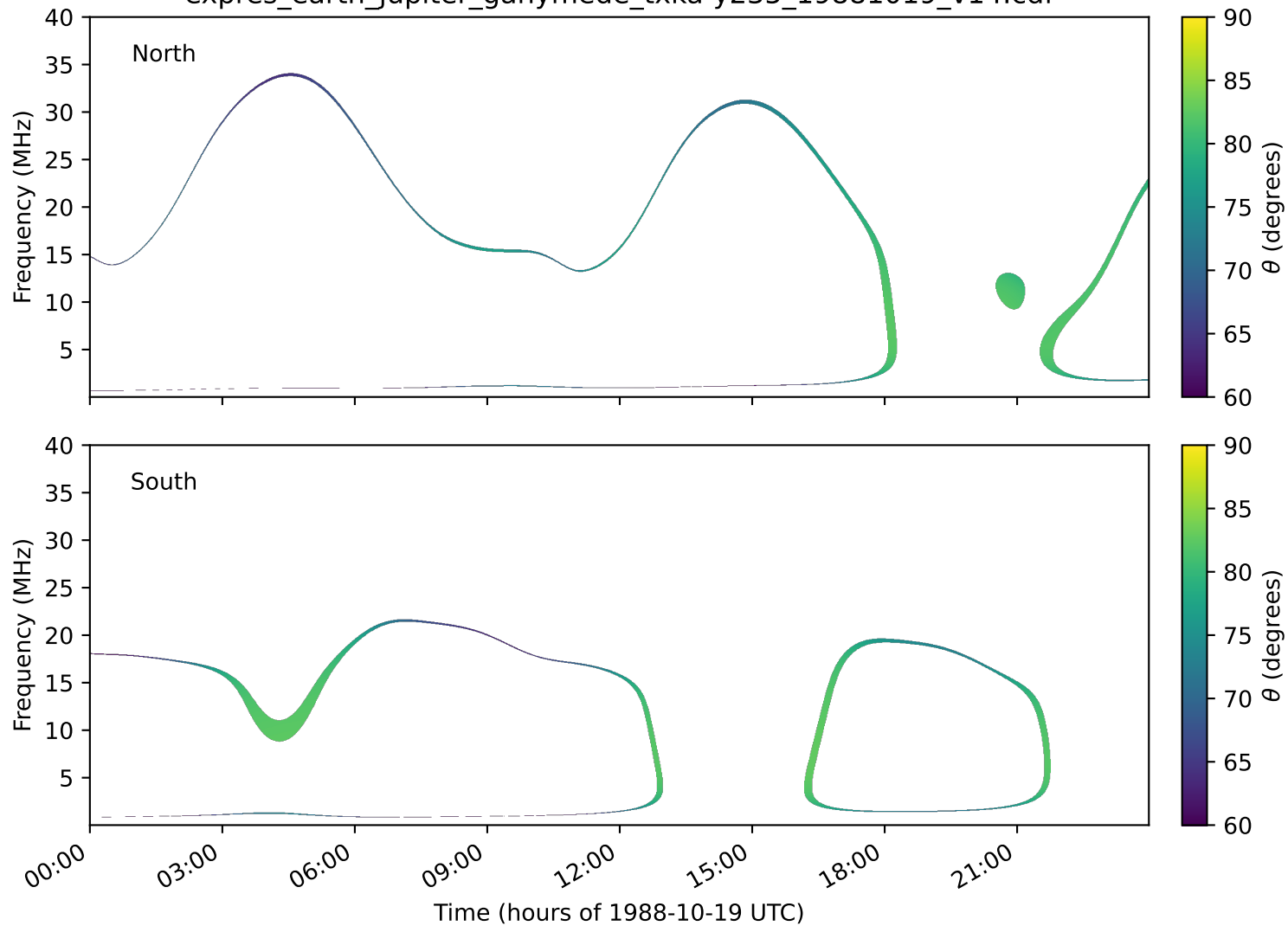
expres_earth_jupiter_ganymede_txka-y235_19881019_v14.cdf
